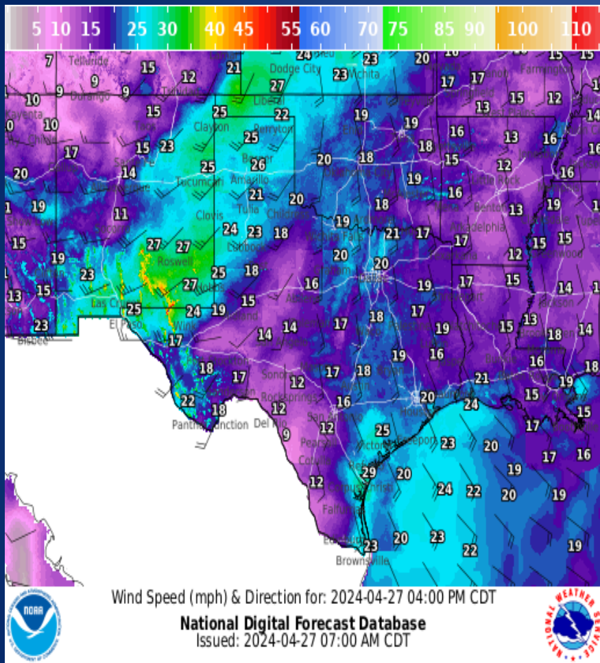
Wind Speeds
